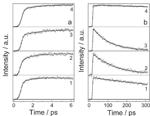
Figure 5. Picosecond fluorescence dynamics of HMBA (1), MBA − (2), H 2 SA (3) and HSA − (4) on the 0–6 ps (a) and 0–300 ps (b) time scales
