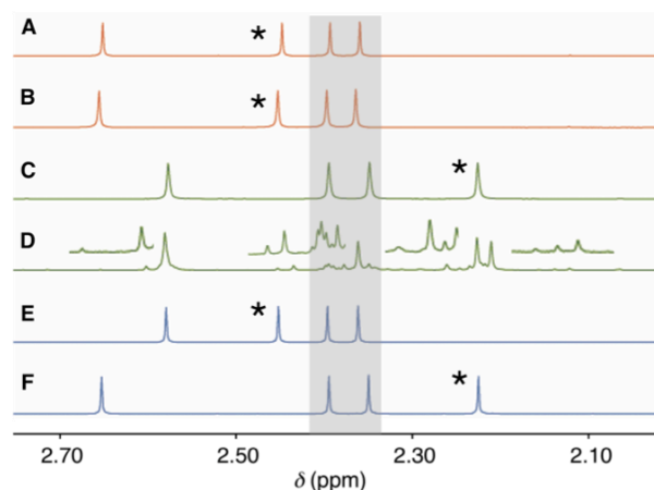
Figure 2. Part of the 1 H NMR spectra of 2 (A; re-measured after 6 days, B), 5 (C; re-measured after 6 hours, D), 4 (E) and 3 (F). The signals of the methyls next to sulfide (*, A, B, E) and methoxy substituents (*, C, F) and the region of those in the middle of the chromophores (grey area) are highlighted. D: Peak patterns from degradation side products are reproduced in magnified form just above the original spectrum.
