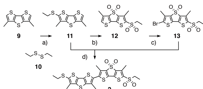
Scheme 1. a) 1. LDA, THF, -78 °C, 30 min; 2. 10 , THF, rt, 12 h, 70%; b) mCPBA, CH 3 Cl, rt, 12 h, 53%; c) NBS, AcOH, CH 2 Cl 2 , reflux, 24 h, 66%; d) 1. LDA, SnCl(Bu) 3 , THF, -78 °C, 1 h; 2. Pd(PPh 3 ) 4 , DMF, 70 °C, 2 d, 38%.
