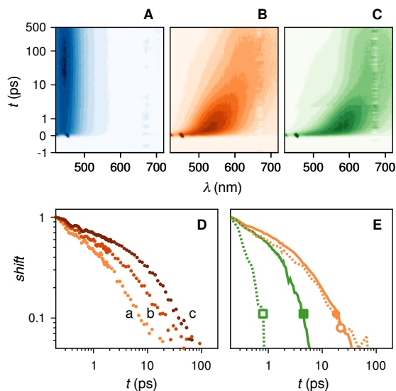
Figure 4. Time-resolved broadband emission spectra of 12 (A), 2 (B) and 3 (C) in EtOAc. (D) Normalized shift of the position of the emission maximum with time, \text{shift} = [\nu(t) - \nu(\infty)] / [\nu(0.2\text{ps}) - \nu(\infty)] , with \nu being the frequency of the fluorescence maximum, 19b after excitation at 400 nm (100 fs pulse) for 2 in alkanes of different viscosity (a, n -hexane, 0.3 cP; b, c -hexane, 0.9 cP; c, n -hexadecane, 2.8 cP). (E) Same for 2 (○, ●) and 3 (□, ■) in solvents of different polarity (ethyl acetate (●, ■), cyclohexane (○, □)).
