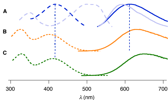
Figure 3. Absorption (left) and emission spectra (right) of 1 (A), 2 (B) and 3 (C) in EtOAc and 1 in solid-ordered membranes (DPPC vesicles at 25 °C; A, light blue). Spectra in A are from ref. 6.
