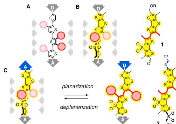
Figure 1. (A) Planarizable push-pull probes, designed to report on lateral pressure and parallel potentials with shifts in excitation. (B) Fluorescent flippers, i.e., large and shiny monomers, added to maximize mechanosensitivity and lifetime ( R = -\text{COCH}_2\text{OCH}_2\text{COOH} ). (C) The concept of turn-on sulfide \pi donors (blue).
