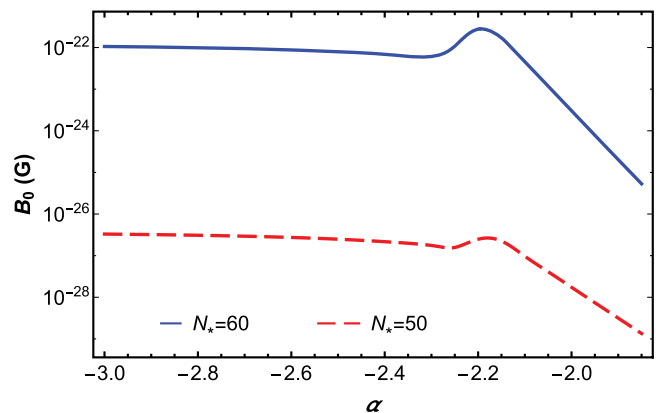
FIG. 4. The dependence of the present-day value of the magnetic field on parameter \alpha for two numbers of e -folds from the moment of the pivot scale horizon crossing to the end of inflation, N_* = 50 (red dashed curve) and N_* = 60 (blue solid curve).
