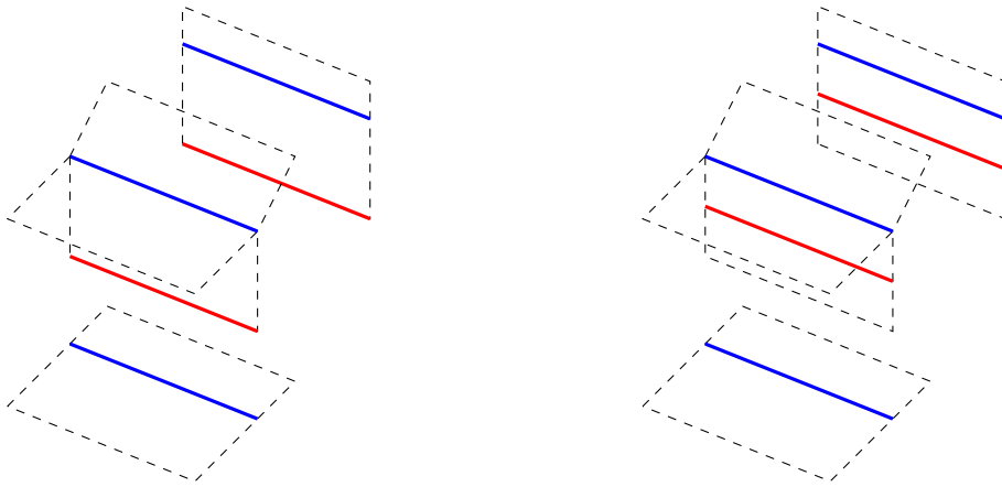
Figure 3.4: Example of a modification of a line along itself. Let L_1, L_2 be defined by y = t^{-1}, y = t^{-1} + t^3 respectively. On the left we see the modification of L_1 along L_1 , on the right we see the modification of L_2 along L_1 . Red line is the result of the modification.
