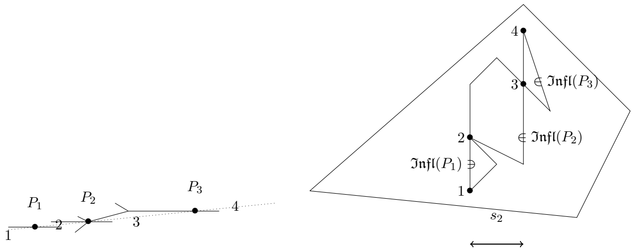
Figure 2.2: The left picture represents a part of a tropical curve through points P_1, P_2, P_3 on an almost horizontal line. The second picture is dual to the first picture, we see parts of the regions of influence of the points P_1, P_2, P_3 . The marked points 1, 2, 3, 4 represent the monomials which are maximal on the parts of the dotted line on the left picture. The lattice path 1, 2, 3, 4 is non-decreasing by the x -coordinate, therefore \sum_{i=1}^n s_i \leq \omega_{(1,0)}(\Delta) .
