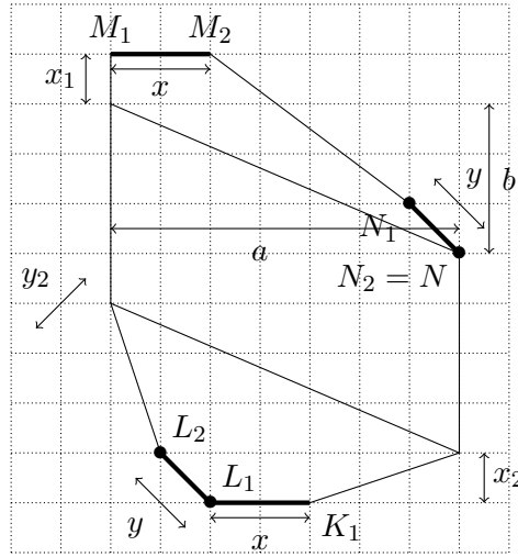
Figure 1.5: In this example m = 11, a = 7 , and y_1 = 0 (therefore N = N_2 ). The vertices MNKL are as in Figure 1.4, left, the vertices M_1M_2, K_1, K_2 are as in Figure 1.4, right, and L_1 and K_2 coincide. We are looking for the minimum of the sum of the area of this polygon and \frac{1}{2}(x^2 + y^2) .
