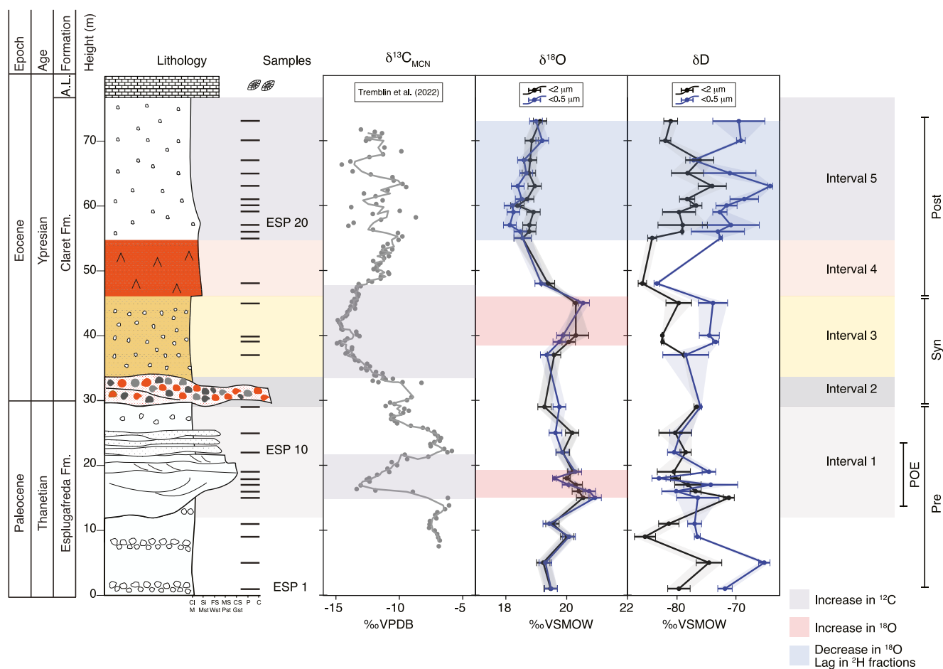
Figure 3. Stable isotope climatic proxies. The carbon isotopes from Tremblin et al. (2022) mark the different sections of the PETM. The \delta D and \delta^{18}O were measured in two size fractions, <0.5 and <2 \mu m . The confidence interval for \delta^{18}O constitutes the analytical uncertainty ( 0.2\text{‰} ) and that of \delta D constitutes the sample replicate reproducibility.
