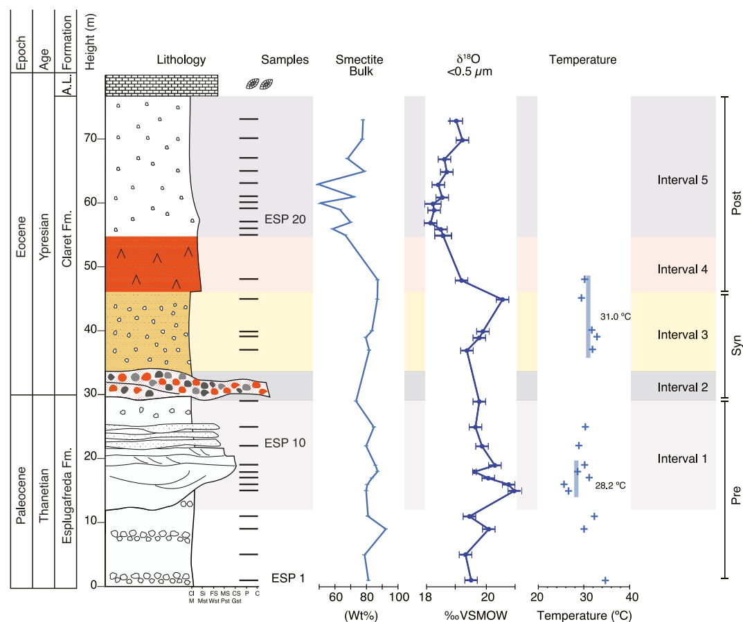
Figure 5. Single-mineral geothermometer from Delgado and Reyes (1996) calculated with the \delta^{18}\text{O} and \delta\text{D} measured in clays (<0.5 \mu\text{m} fraction) for bulk clays containing more than 80% smectite. From left to right, lithology, smectite content through the section, \delta^{18}\text{O} smectite of the <0.5 \mu\text{m} clay fraction, and crystallization temperature calculated with Equation 6. For the POE, we calculated a relative error of 1.0°C, a standard deviation of 2.1°C, and an average Monte Carlo error propagation of 3.0°C. For the Syn-PETM, we calculate a relative error of 0.8°C, a standard deviation of 1.3°C, and an average Monte Carlo error propagation of 2.5°C.
