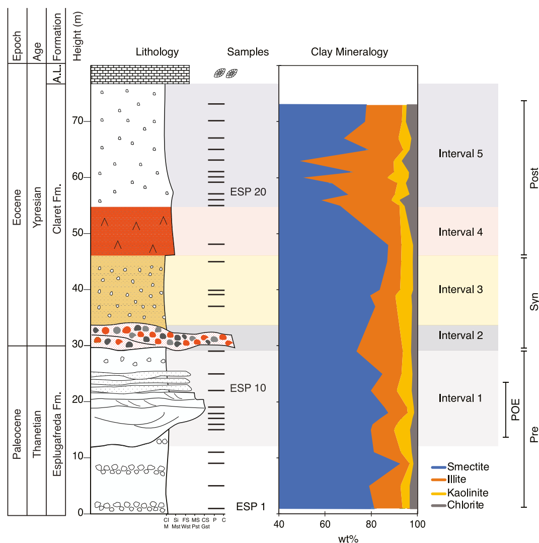
Figure 2. Esplugafreda section cumulative clay mineralogy. The clay mineralogy assemblage is dominated by smectite throughout the section, with a constant amount during the Pre- and Syn-PETM (intervals 1 and 3) and a decrease in smectite during the Post-PETM (intervals 4 and 5). Illite, kaolinite, and chlorite are present in minor amounts, peaking during intervals 4 and 5.
