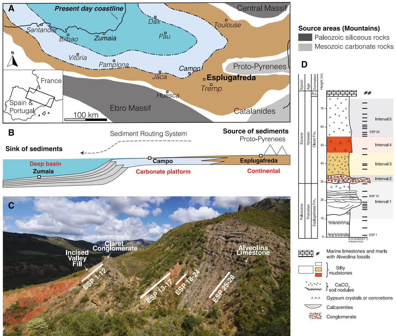
Figure 1. (a) Location of the study section (map of Spain) and paleogeography during the late Paleocene and early Eocene. Redrawn and modified from Pujalte et al. (2016). (b) Sediment routing system, modified from Tremblin et al. (2022). (c) Sampling divided into four transects. (d) Stratigraphy, modified from Khozyem (2013) and Pujalte et al. (2009) and sample distribution.
