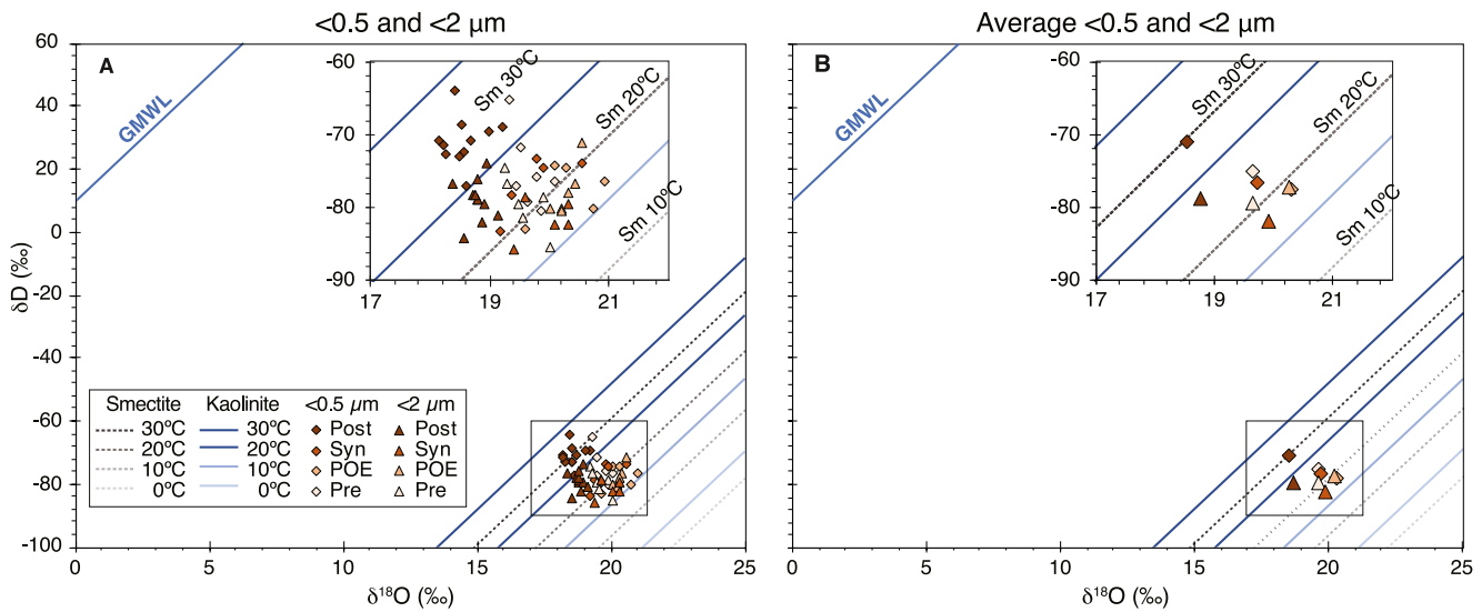
Figure 4. Cross plots of the \delta D versus \delta^{18}O of clays, color, and symbol coded according to the different intervals described. (a) Presents all the data points in both size fractions, and (b) displays the average isotopic composition in each interval for each size fraction. Data points in the two size fractions are coded according to the period relative to the PETM. Global Meteoric Water Line (GMWL) and isotherms for kaolinite and smectite at 0, 10, 20, and 30°C from Sheppard and Gilg (1996) and Yeh (1979). The kaolinite isotherms have a lower \delta^{18}O for the same crystallization temperatures. Hence, the cluster of the Post-PETM to the left of the Syn- and Pre-PETM clusters reflects a change in the mineralogy. (b) Average values in each size fraction for the four periods.
