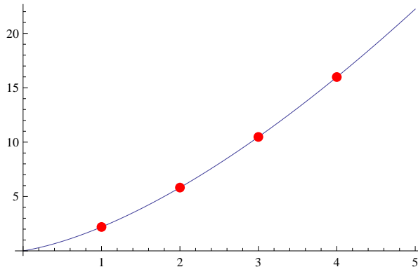
Figure 4: The smooth line gives the free energy F(N, 2\pi) of local \mathbb{P}^2 as a function of N , computed from (3.43), while the points give the values of the free energy as computed from the spectral traces (4.23).
