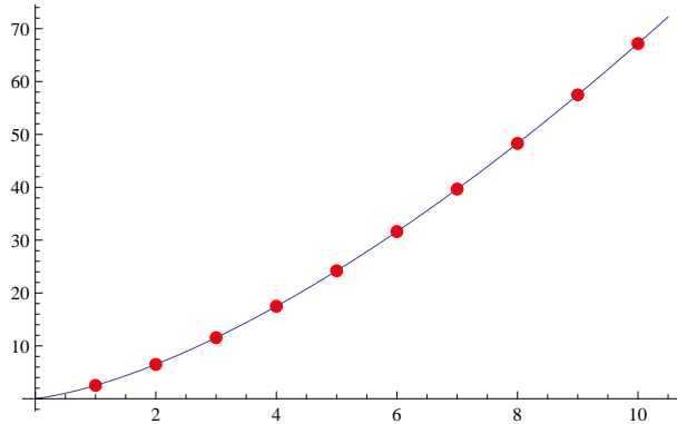
Figure 5: The smooth line gives the free energy F(N, 2\pi) of local \mathbb{F}_1 as a function of N , computed from (3.43), while the points give the values of the free energy as computed from the spectral traces.
