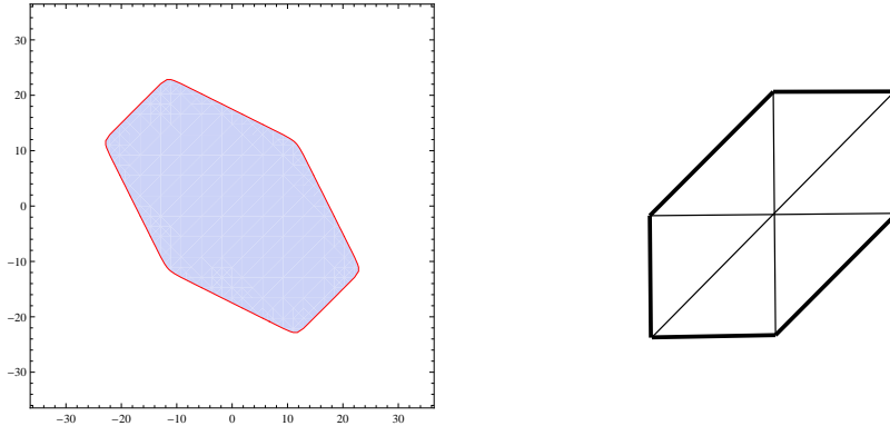
Figure 2: The figure on the left shows the region (2.39) in phase space for the quantum operator associated to local \mathcal{B}_3 , for E = 35 and m_1 = m_2 = m_3 = 1 . The figure on the right is the polyhedron representing toric \mathcal{B}_3 .
