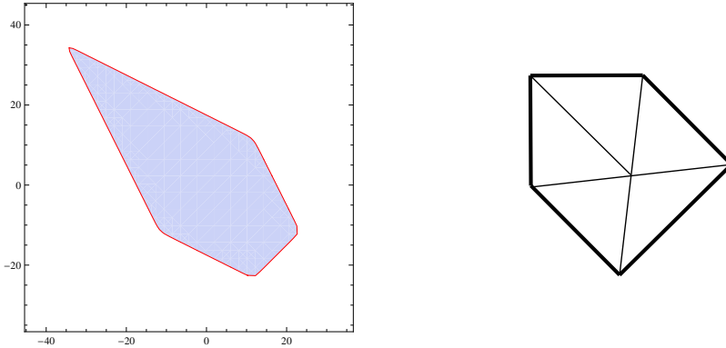
Figure 1: The figure on the left shows the region (2.39) in phase space for the quantum operator associated to local \mathcal{B}_2 , for E = 35 and m_1 = m_2 = 1 . The figure on the right is the polyhedron representing toric \mathcal{B}_2 .
