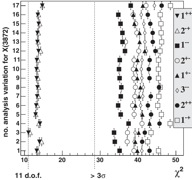
FIG. 4. Total \chi^2 for different analysis variations on the y-axis, explained in the text. Vertical bars are added for visual guidance. The \chi^2 values of the spin 0 states are all above 100. The 2^{--} and 3^{--} states have the same angular distribution as the 1^{+-} state.
