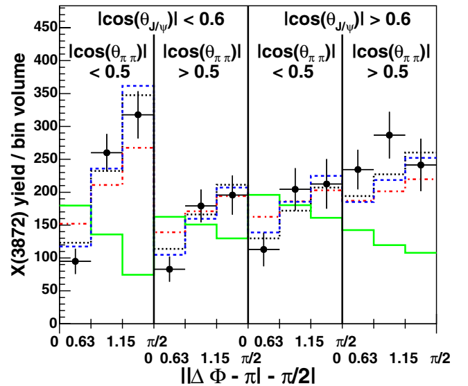
FIG. 3 (color online). Measured 3D angular distribution with acceptance corrected predictions for J^{PC} = 0^{++} (solid line), 1^{++} (dotted line), 2^{-+} (dashed line), and 1^{--} (dash-dotted line). The plot is divided into 2 \times 2 regions, corresponding to intervals of |\cos(\theta_{J/\psi})| and |\cos(\theta_{\pi\pi})| . Each region shows the distribution of ||\Delta\Phi - \pi| - \frac{\pi}{2}| in 3 bins. The bin contents have been scaled to the same bin volume.
