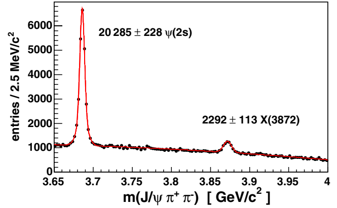
FIG. 1 (color online). The J/\psi \pi^+ \pi^- mass spectrum after optimizing the selection cuts, fitted by a double Gaussian function for the \psi(2S) (left), a Gaussian function for the X(3872) particle (right), and a second order polynomial for the combinatorial background.
