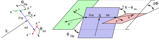
FIG. 2 (color online). Definition of the decay angles. The polar angles ( \theta ) are calculated from the parent momenta and the child momenta in the corresponding parent rest frame.
