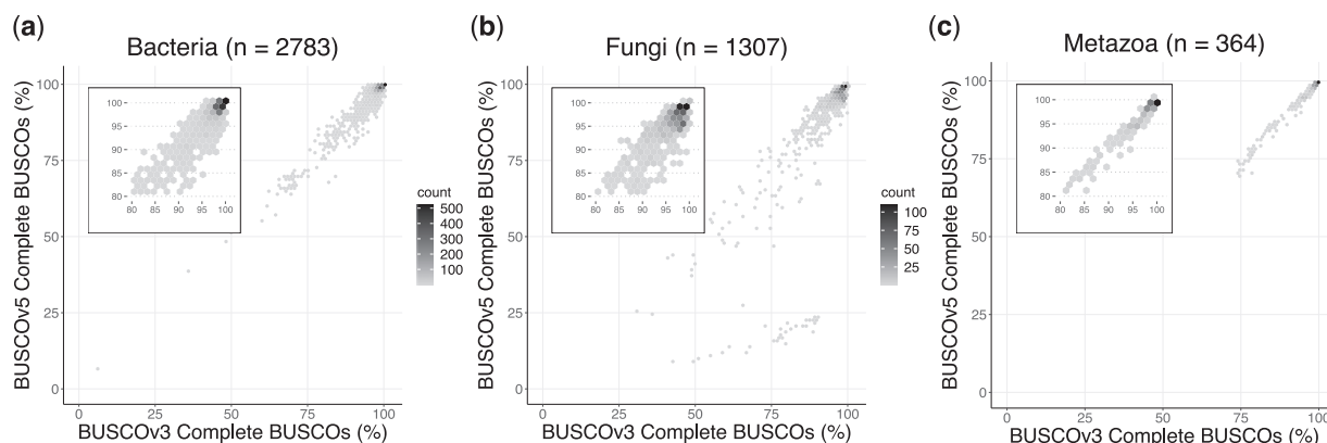
FIG. 1. Comparison of the number of complete BUSCOs obtained by running BUSCO v5 and v3 with BUSCO odb_10 and odb_9 data sets on (a) bacterial, (b) fungal, and (c) metazoan gene sets.
