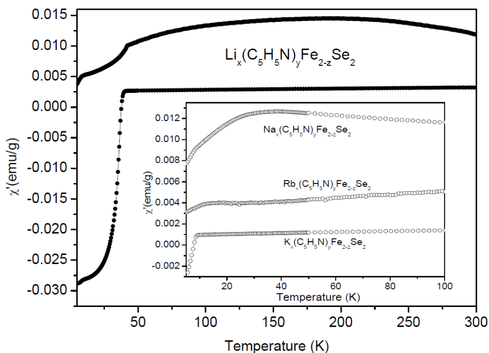
Figure 4. Temperature dependence of the real part of the ac magnetic susceptibility for \text{A}_x(\text{C}_5\text{H}_5\text{N})_y\text{Fe}_{2-z}\text{Se}_2 samples. The upper curve corresponds to a \text{Li}_x(\text{C}_5\text{H}_5\text{N})_y\text{Fe}_{2-z}\text{Se}_2 pristine sample, the lower one to \text{Li}_x(\text{C}_5\text{H}_5\text{N})_y\text{Fe}_2\text{Se}_2 sample post-annealed at 215 °C. In the insert the real part of the ac magnetic susceptibilities for \text{A}_x(\text{C}_5\text{H}_5\text{N})_y\text{Fe}_{2-z}\text{Se}_2 ( \text{A}=\text{Na} , \text{Rb} and \text{K} ) samples are presented.
