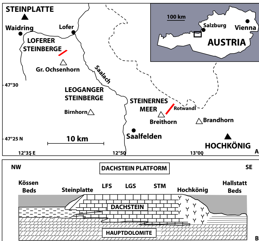
FIGURE 1 (A) Location of the measured sections in Steinernes Meer and Loferer Steinberge (respective bars) southwest of Salzburg, Austria. (B) Stratigraphic sketch of the Dachstein platform and the adjacent basins. LFS, Loferer Steinberge; LGS, Leoganger Steinberge; STM: Steinernes Meer
