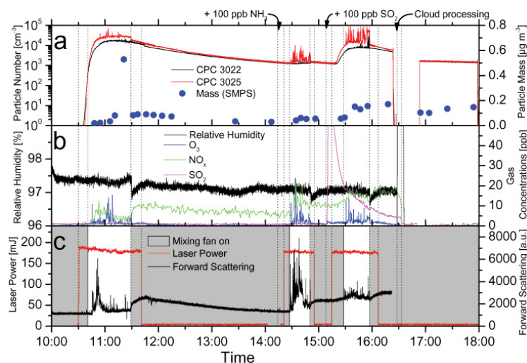
Fig. 6. Particle and trace gas formation by laser filaments in the synthetic air for experiments 5 and 8 at 283 K and 97 % RH. The panels show (a) particle number (red and black line) and mass (blue circles); (b) relative humidity (black line), ozone (blue line), NO x (green line), and SO 2 concentrations (magenta line); (c) near forward scattering (black line), laser power (red line) and mixing fan operation (grey shaded area).
