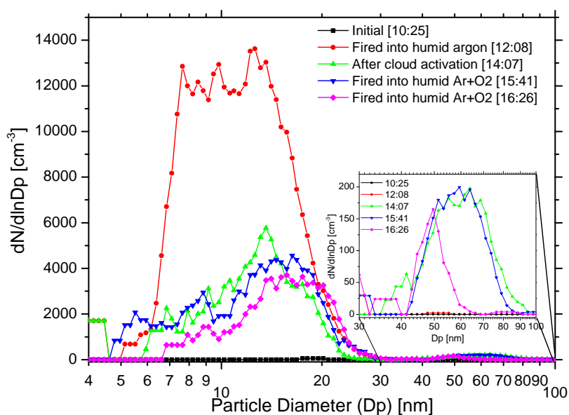
Fig. 3. Particle size distributions for selected times during experiments 1 and 2 in pure argon and in an argon-oxygen mixture (15 % O _2 ) at 283 K and at 64 % as well as 55 % relative humidity, respectively. Times in the legend refer to Fig. 2.
