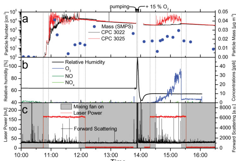
Fig. 2. Particle and trace gas formation by laser filaments for experiments 1 and 2 in pure argon and in an argon-oxygen mixture (15 % O _2 ) at 283 K and at 64 % as well as 55 % relative humidity, respectively. The panels show (a) aerosol particle number (black and red lines) and mass concentrations (blue circles); (b) relative humidity (black line), ozone (blue line), NO (dark green line), and NO _x concentrations (light green line); (c) as well as near-forward scattering (black line), laser power (red line) and mixing fan operation (shaded grey area). Dashed vertical lines indicate the time of events like switching on/off the laser, the fan, or a pump.
