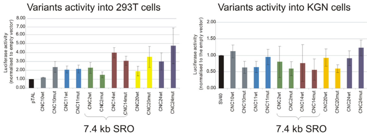
Figure 4. Regulatory activity of wild-type and variant CNCs in FOXL2 expressing and non-expressing cells. The 25 identified CNCs and their putative pathogenic variants were cloned into a luciferase reporter vector and assayed for their regulatory role into expressing KGN and non-expressing 293T (human kidney cells) cells. (A) Bar chart showing the regulatory activity of each independent wild type CNC (CNCwt) in KGN (brown bars) and 293T (blue bars) relative to the basal activity of the empty vector (pTAL). Significant changes (one sample T-test, p value < 0.05 ) are highlighted by an asterisk. CNCs with a > 2 fold-change in activity between cell lines and a significant p value are shown in red. (B) Bar chart of wtCNCs and variant CNCs (CNCmut) regulatory activity in 293T and KGN cell lines respectively. Each CNC activity is first normalised to the basal activity of the empty vector and significant changes between wt and mut were then assessed by a two-samples T-test. No significant p values were found for any assayed construct ( P value < 0.05 ). doi:10.1371/journal.pgen.1000522.g004
