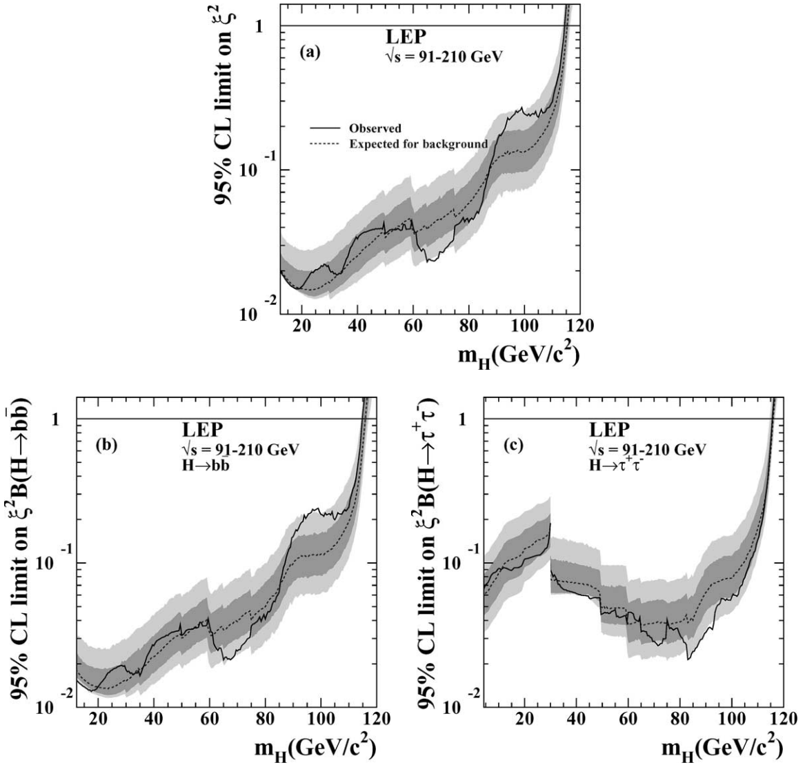
Fig. 10. The 95% confidence level upper bound on the ratio \xi^2 = (g_{HZZ}/g_{HZZ}^{\text{SM}})^2 (see text). The dark and light shaded bands around the median expected line correspond to the 68% and 95% probability bands. The horizontal lines correspond to the Standard Model coupling. (a): For Higgs boson decays predicted by the Standard Model; (b): for the Higgs boson decaying exclusively into b\bar{b} and (c): into \tau^+\tau^- pairs.
