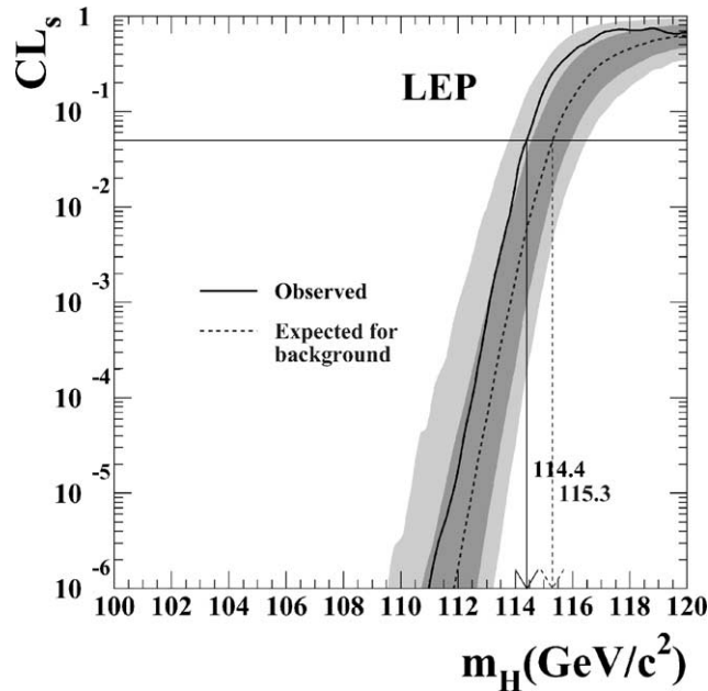
Fig. 9. The ratio CL_s = CL_{s+b}/CL_b for the signal plus background hypothesis, as a function of the test mass m_H . Solid line: observation; dashed line: median background expectation. The dark and light shaded bands around the median expectation for the background hypothesis correspond to the 68% and 95% probability bands. The intersection of the horizontal line for CL_s = 0.05 with the observed curve is used to define the 95% confidence level lower bound on the mass of the Standard Model Higgs boson.
