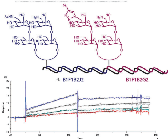
Fig. 3 Affinity of three assemblies for DC-SIGN measured by SPR. Top: calculated K_D of three assemblies in two buffers (the letters denote the fragments, see Fig. 1 for the structure); Middle: structure of assembly 4 identified in the screen, sensogram of assembly 4 at 25, 12.5, 6.25 and 3.12 \mu\text{M} (entry 1).
