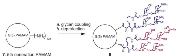
Fig. 4 Synthesis of a glycodendrimer 8 derivatized with glycan fragments of assembly 4 .
