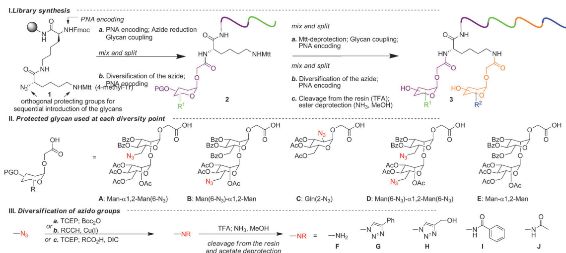
Fig. 1 Split and mix synthesis of a PNA-encoded library of glycans.
