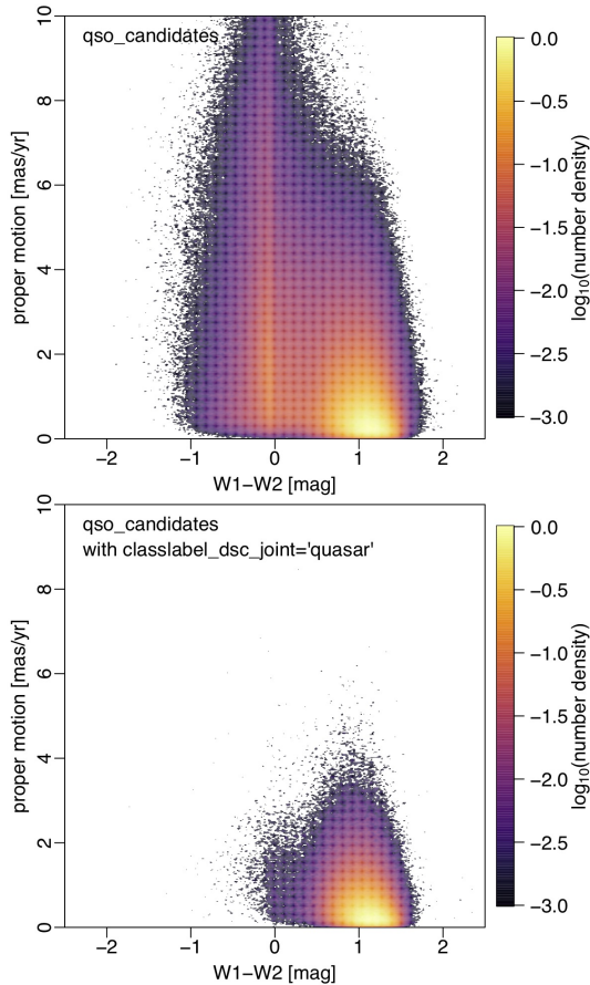
Fig. 28. Gaia proper motion vs. catWISE W1-W2 colour for all sources in the qso_candidates table (top) and the subset with classlabel_dsc_joint = quasar (bottom). Regions around the LMC and SMC are excluded. The colour scale shows the density of sources on a log scale relative to the peak density (densities 1000 times lower than the peak are not shown).
