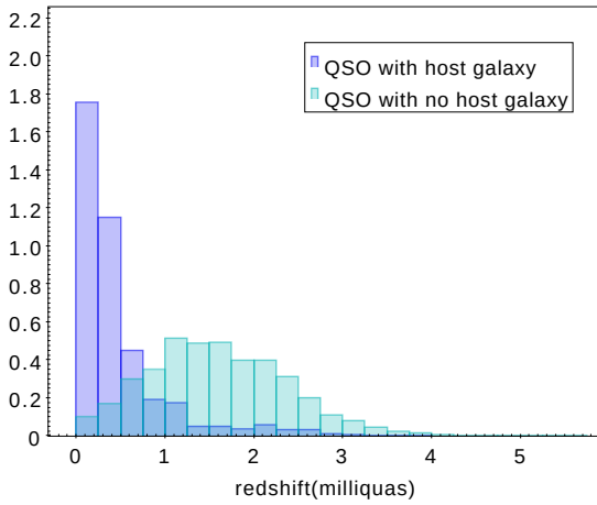
Fig. 13. Normalized distribution of the redshifts from Milliquas v7.2aa (Flesch 2021) of quasars that were analysed for surface brightness profiles. Blue shows the 2000 quasars for which a host galaxy was detected by Gaia , and turquoise the remaining 224 000 quasars for which no host galaxy was detected.
