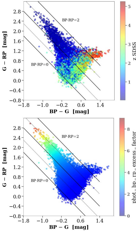
Fig. 31. Colour-colour diagram for the set in Fig. 30 colour-coded by redshift (top) and Gaia phot_bp_rp_excess_factor (bottom). The straight lines correspond to fixed G_{BP}-G_{RP} colour, with values 2, 1.5, 1, 0.5 and 0.
