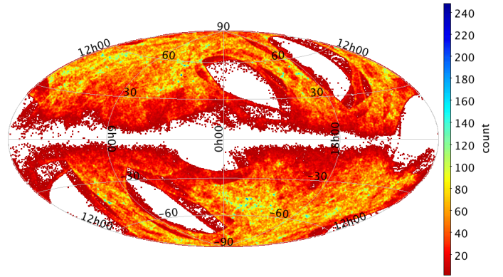
Fig. 15. Distribution in Galactic coordinates (Hammer-Aitoff projection) of the galaxies processed by the surface brightness profile module. The colours show the density on a linear scale.
