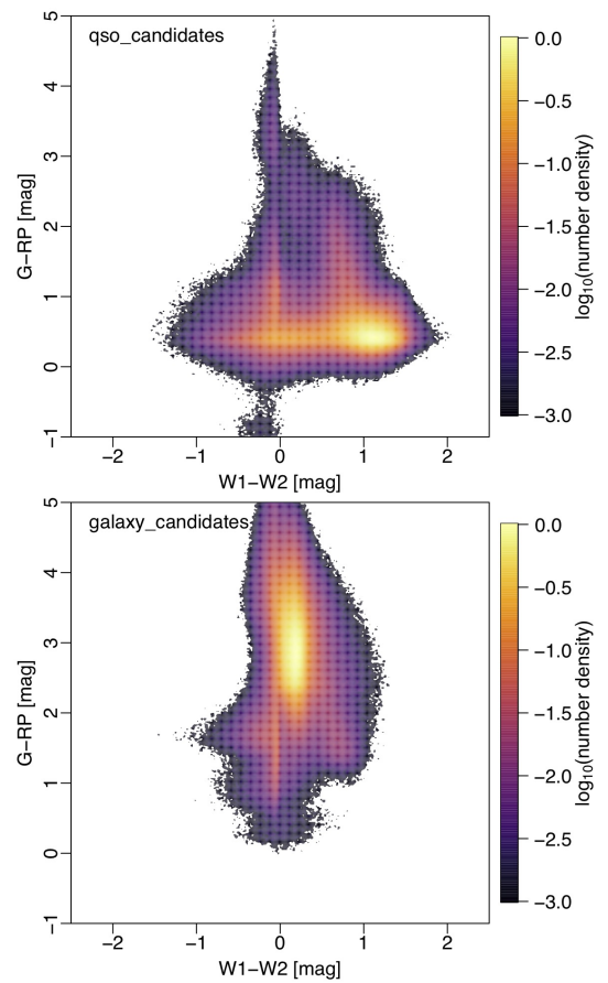
Fig. 27. Gaia - catWISE colour-colour diagrams. Top : all sources in the qso_candidates table. Bottom : all sources in the galaxy_candidates table. In both cases regions around the LMC and SMC have been excluded. The colour scale shows the density of sources on a log scale relative to the peak density (densities 1000 times lower than the peak are not shown).
