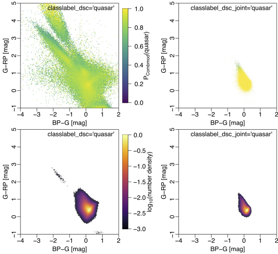
Fig. 8. Colour-colour diagram for sources in the qso_candidates table, excluding regions around the LMC and SMC. Left column: shows sources with classlabel_dsc=quasar (2.77 million sources), the right column: shows sources with classlabel_dsc_joint=quasar (the purer subset, 0.52 million sources). These numbers refer to the number of sources plotted, which are those that have all Gaia bands. Upper panel: mean DSC-Combmod probability for the quasar class (the field classprob_dsc_combmod_quasar ). Lower panel: density of sources on a log scale relative to the peak density in that panel (densities 1000 times lower than the peak are not shown).
