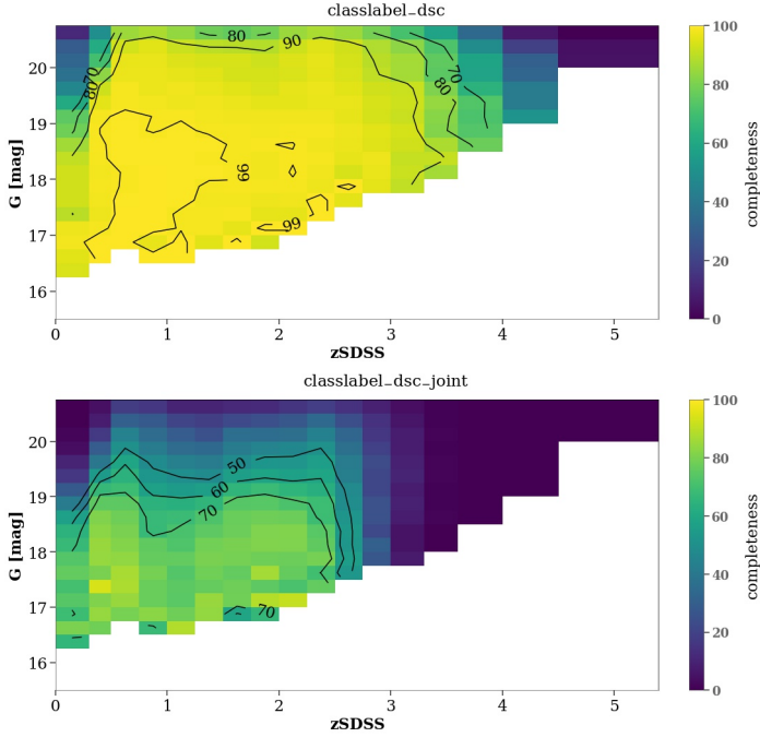
Fig. 29. Completeness of classlabel_dsc=quasar (top) and classlabel_dsc_joint=quasar (bottom) with respect to the SDSS-DR14Q-Gaia DR3 cross-match as a function of G and SDSS redshift. Empty bins (white) have fewer than 25 sources.
