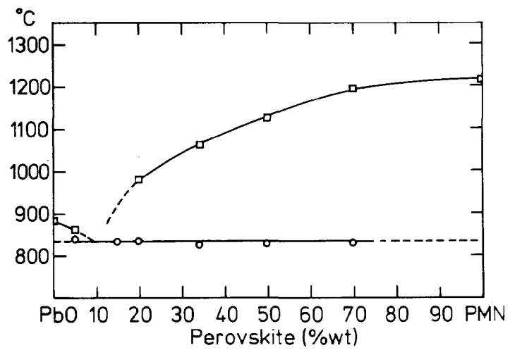
Fig. 4. The PbO—PMN phase diagram.
