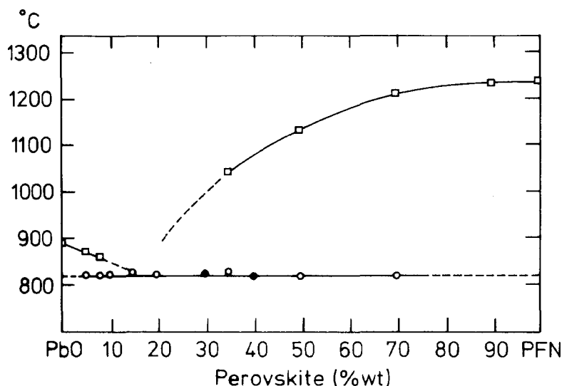
Fig. 3. The \text{PbO} —PFN phase diagram. The filled circles indicate the measurements made with the less sensitive platinum tube crucible form.
