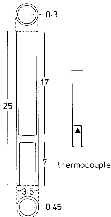
Fig. 1. The platinum sample crucible. The dimensions are in mm.
