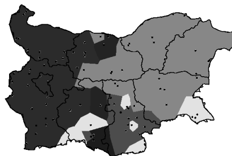
Figure 2: Classification map
