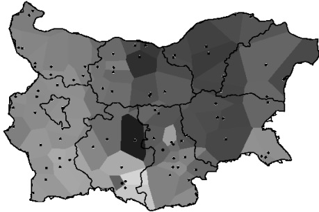
Figure 3: MDS map
