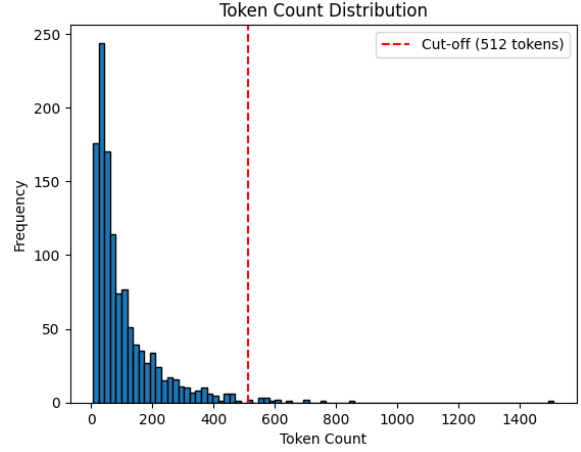
Figure 1: Token Count Distribution in the Dialogues.
