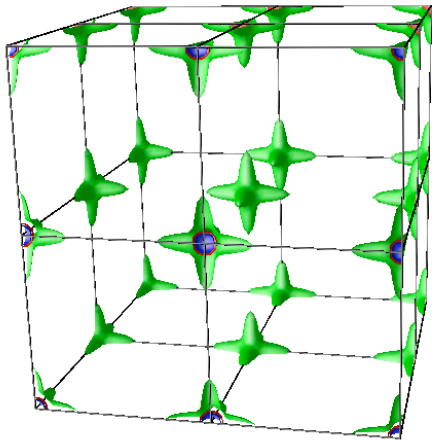
FIG. 4: Fermi surface of the high-temperature cubic phase at 2% doping, showing the large anisotropy of the lowest band. At the critical doping x_c = 0.097 a topological transition takes place where the Fermi surfaces open up along the three axis.
