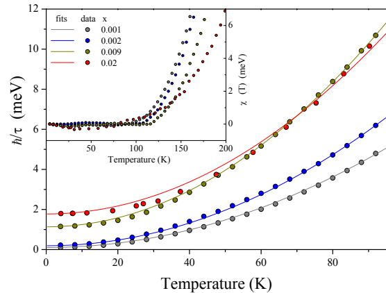
FIG. 2: Temperature dependent relaxation rates of SrTi 1-x Nb x O 3 for 4 different carrier concentrations, using the relation \rho(T) = 4\pi\omega_p^{-2}\tau^{-1} . Plasma-frequencies, \omega_p , are obtained from the Drude spectral weight measured with infrared spectroscopy 34 and listed in table II. Inset: Difference between experimental data and fitted curve, \chi(T) = \hbar/\tau(T) - \hbar/\tau_{fit}(T) , demonstrating upward departure from T^2 behavior of the resistivity above 100 K.
