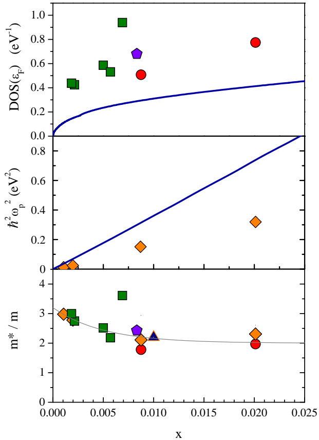
FIG. 6: Top panel: Doping dependence of the density of states (DOS) at the Fermi energy. The solid curve corresponds to the tight-binding bandstructure fitted to the Wien2k ab initio bandstructure, with parameters of the first row of table IV. Squares 42 , circles 33,43 , pentagon 44 : Density of states obtained from the linear term in the specific heat. Middle panel: Doping dependence of the Drude spectral weight, \omega_p^2 . The solid curve corresponds to the bandstructure results. Diamonds are the experimental values 34 . Bottom panel: (i) Ratio of experimental DOS over bandstructure DOS (experimental and theoretical values taken from top panel, the meaning of the symbols is the same). (ii) Ratio of bandstructure over experimental \omega_p^2 (values taken from middle panel). (iii) Ratio of bare and experimental (dressed) Fermi-velocity, v_{F,b}/v_{F,e} (triangle, data from Ref. 37). The grey curve is a smooth interpolation, m^*/m_b = 2.0 + 1.2 \exp(-x/0.005) .
