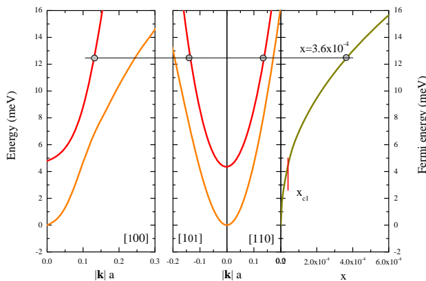
FIG. 5: Enlarged view of Fig. 3 indicating the position of the Fermi level for x = 3.6 \cdot 10^{-4} charge carriers. The corresponding value ka = 0.134 is in excellent agreement with the hitherto unexplained de Haas-van Alphen frequency reported by Gregory et al. 41 .
