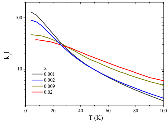
FIG. 7: The quantity k_F l where l is the mean free path, calculated using k_F l = 2\epsilon_F^* \hbar^{-1} \tau , and using the experimental \tau of Fig. 2 and the calculated Fermi energies corrected by the mass renormalization of Fig. 6. The high values of k_F l below 100 K imply the itinerant character of the charge carriers.
