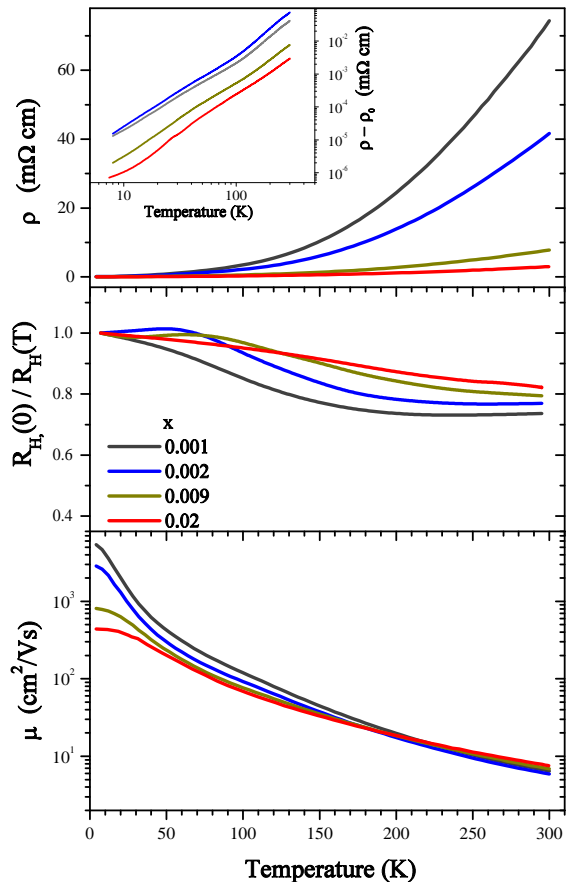
FIG. 1: Temperature dependence of the resistivity, the inverse Hall constant and the mobility of \text{SrTi}_{1-x}\text{Nb}_x\text{O}_3 for different carrier concentrations.
