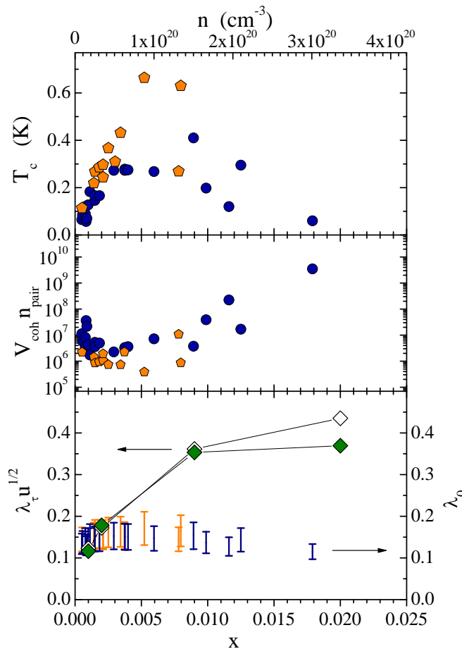
FIG. 8: Top panel: T_c of a large number of samples. Pentagons: data by Binnig et al. 4 . Circles: data by Koonce et al. 3 . Middle panel: Coherence volume times the density of Cooper pairs. The high value indicates that each pair is overlapping with a huge number of other pairs. Lower panel: Doping dependence of the coupling constants \lambda_\tau obtained from the T^2 term of the resistivity and \lambda_0 from T_c . Circles: \lambda_\tau using a_2 listed in the second column of table II and Eq. 3. Diamonds: idem using a'_2 . Bars: coupling constants \lambda from T_c at the corresponding carrier concentration of \text{SrTi}_{1-x}\text{Nb}_x\text{O}_3 using the T_c 's of the top panel and Eq. C5, \epsilon_F^* = \epsilon_F m_b / m^* using \epsilon_F from Fig. 3 and m^*/m_b from Fig. 6. Upper (lower) limits of the bars indicate the value for g obtained with \omega_c = 5 meV (80 meV).
