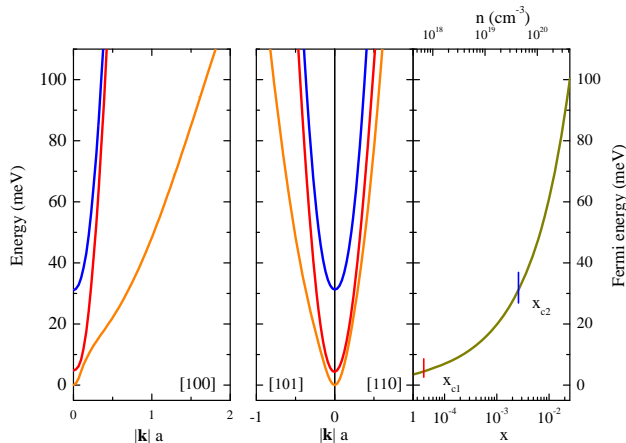
FIG. 3: Band dispersion of the lowest unoccupied bands of SrTiO 3 in the low temperature tetragonal phase. The directions in momentum space are labeled according to the high temperature cubic Brillouin zone, so that [1, 0, 0] corresponds to momentum along the Ti-O bond direction. The rightmost panel indicates the position of the Fermi energy as a function of carrier concentration. x_{c1} = 4.0 \cdot 10^{-5} and x_{c2} = 2.6 \cdot 10^{-3} are critical carrier concentrations where the Fermi energy enters the second and the third band.
