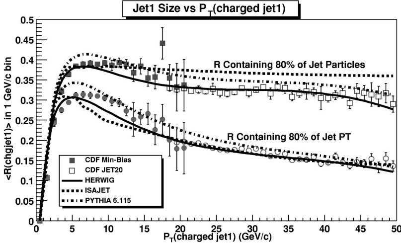
FIG. 6. The average radius in \eta - \phi space containing 80% of the charged particles (and 80% of the charged p_T sum) as a function of the transverse momentum of the leading charged jet compared with the QCD Monte Carlo model predictions of HERWIG, ISAJET, and PYTHIA 6.115. The solid (open) points are min-bias (JET20) data.
