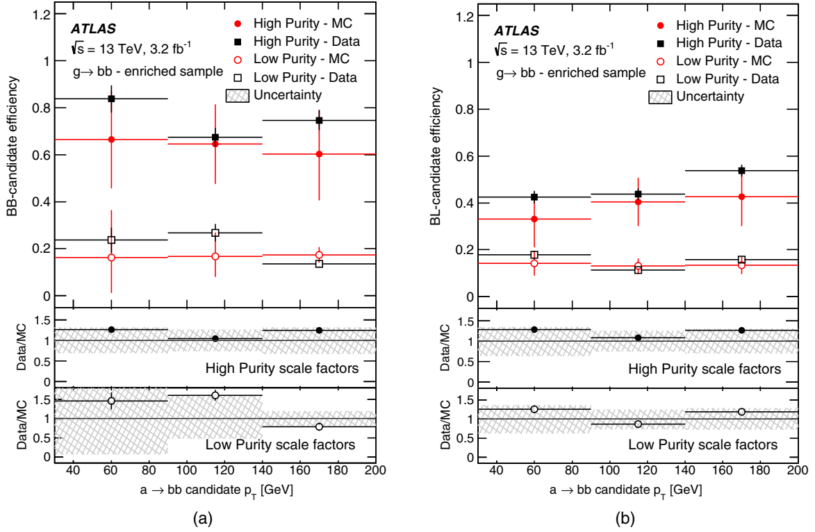
FIG. 4. Efficiency of the a \rightarrow b\bar{b} identification criteria measured in data and simulated multijet events. The efficiency is measured in three transverse momentum ranges, separately for (a) BB and (b) BL candidates in both the HPC and LPC. The ratio of the measured values in data and simulation (bottom panels) are SFs used in the analysis when comparing simulation with data. The error bars in the top panels are statistical only, while the hashed bands on the ratios in the bottom panels include the full systematic uncertainties.
