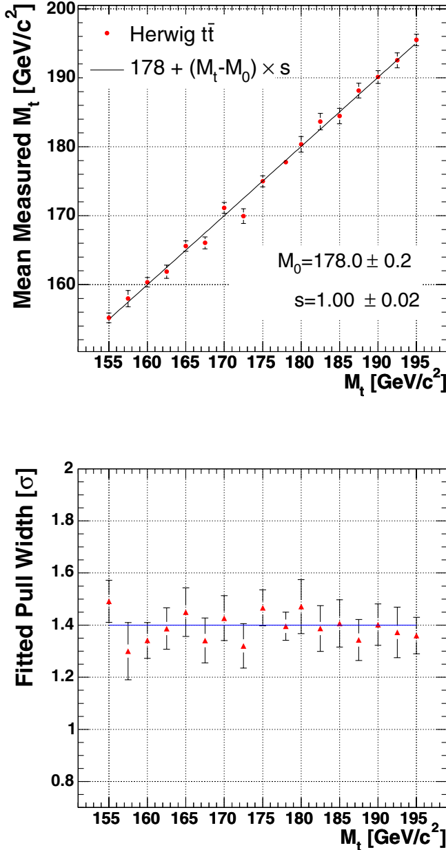
FIG. 4 (color online). Top, mean of measured M_t in Monte Carlo experiments with only t\bar{t} events. Bottom, fitted widths of pull distributions from the same Monte Carlo experiments.
