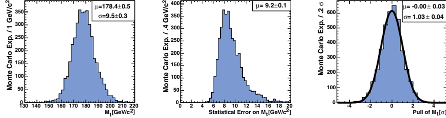
FIG. 9 (color online). Left, distribution of measured M_t in Monte Carlo experiments with t\bar{t} events at M_t = 178 \text{ GeV}/c^2 and background events. Measured statistical error, center, and pull distribution, right, are also shown. All mass and error corrections have been applied.
