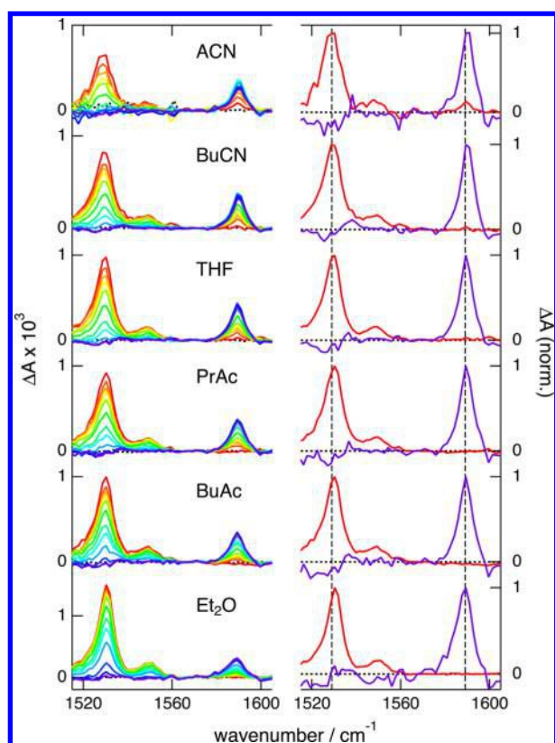
Figure 4. Left column: Transient IR spectra associated with the [-C=C-]^* ( 1531 and 1549 \text{cm}^{-1} ) and [-C=C-]^{*\dagger} ( 1589 \text{cm}^{-1} ) aromatic ring vibrations measured with DMeA/PN after excitation at 400 nm in six different solvents. The concentration of PN was 0.4 M, except for BuAc ( 0.3 M) and Et 2 O ( 0.05 M) (dashed line -30 ps; red to purple lines: 1, 10, 20, 30, 50, 100, 200, 300, 500, 1000, 1500, and 1900 ps). Right column: Corresponding intensity-normalized spectra at 1 ps (red) and 1900 ps (purple).
