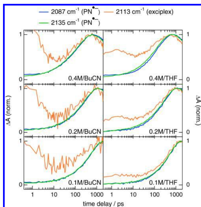
Figure 7. Intensity-normalized time profiles of the transient signal at wavenumbers corresponding to the band maximum of the ions and the exciplex at different PN concentrations in BuCN and THF.
