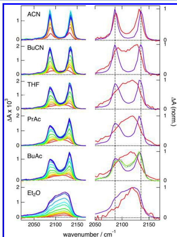
Figure 3. Left column: Transient IR absorption spectra associated with the antisymmetric ^3[-C\equiv N]^{\bullet-} ( 2087\text{ cm}^{-1} ) and symmetric ^5[-C\equiv N]^{\bullet-} ( 2135\text{ cm}^{-1} ) vibrations of the anion PN^{\bullet-} and the [-C\equiv N]^{\delta-} vibration of the exciplex ( 2113\text{ cm}^{-1} ) measured with DMeA/PN after 400 nm excitation in various solvents. The concentration of PN was 0.4 M, except for BuAc (0.3 M) and Et_2O (0.05 M) (dashed line –30 ps; red to purple lines: 1, 10, 20, 30, 50, 100, 200, 300, 500, 1000, 1500, and 1900 ps) Right column: Corresponding intensity-normalized spectra at 1 ps (red) and 1900 ps (purple). Additionally, the normalized spectrum in BuAc at 100 ps (green) is compared with that recorded at 1900 ps with 0.05 M PN (dashed purple).
