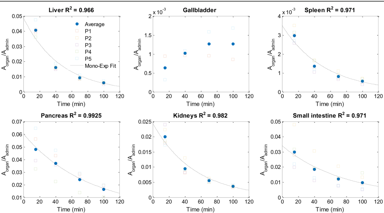
Fig. 2 ^{68}\text{Ga} -NODAGA-MJ9 normalised time-activity curves for most relevant abdominal organs. The organ activity was normalised to the patient administered activity. Coloured squares indicate patient-related data points. Blue dots indicate the normalised activity (mean \pm SD) obtained at each time point. The coefficient of determination ( R^2 ) of the mono-exponential fit (except for the gallbladder, see methods) is reported for each organ. Due to previous surgery, gallbladder and pancreatic normalised time-activity curves were available for two and four patients only, respectively
