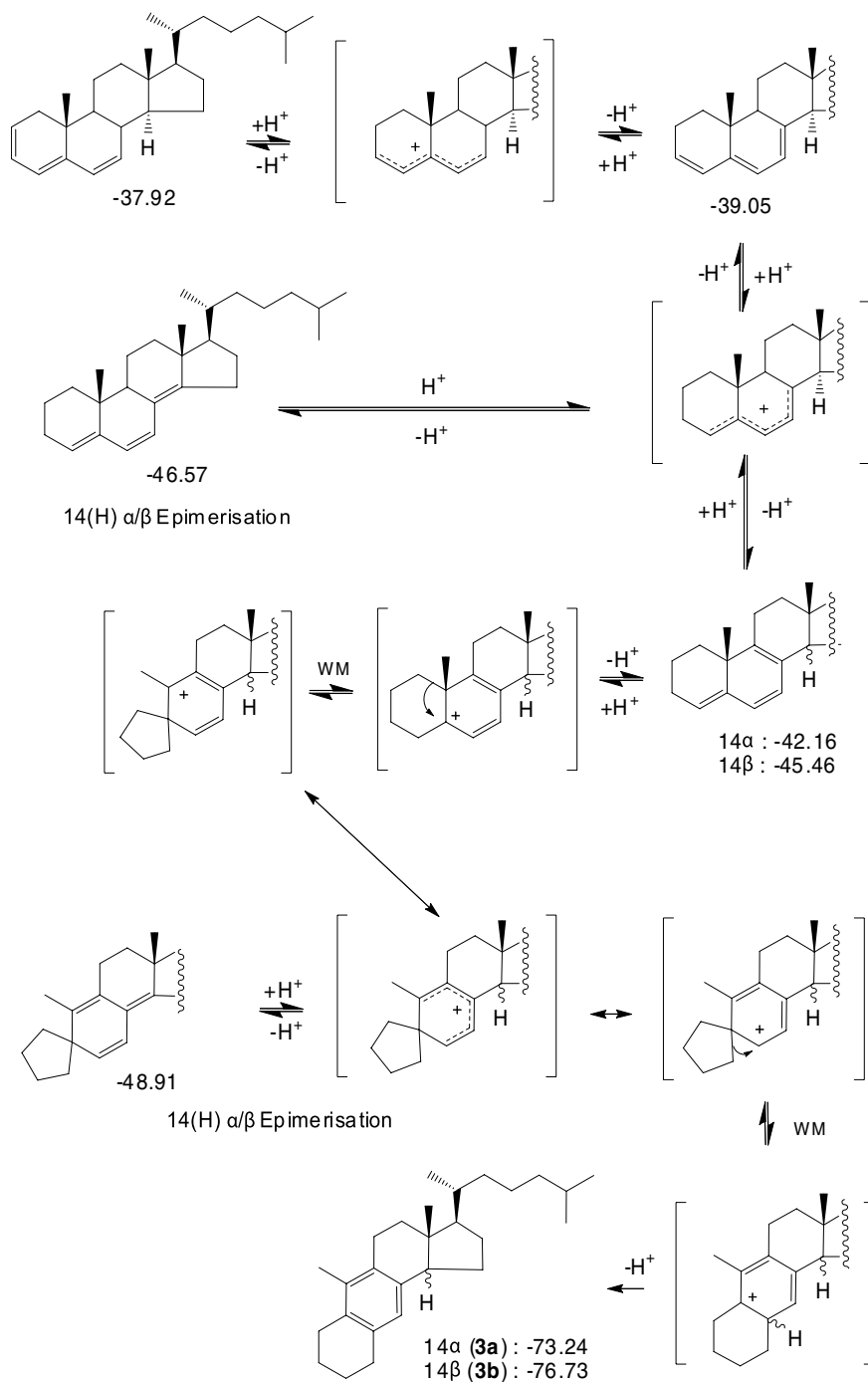
Fig. 6. Proposed formation mechanism of 1(10 \rightarrow 6)-abeo-14 \beta -cholesta-5,7,9(10)-triene ( 3b ) and 1(10 \rightarrow 6)-abeo-14 \alpha -cholesta-5,7,9(10)-triene ( 3a ) from cholesta-2,4,6-triene ( 1 ). Calculated enthalpies of formation (in kcal/mol) are given below the structures.
