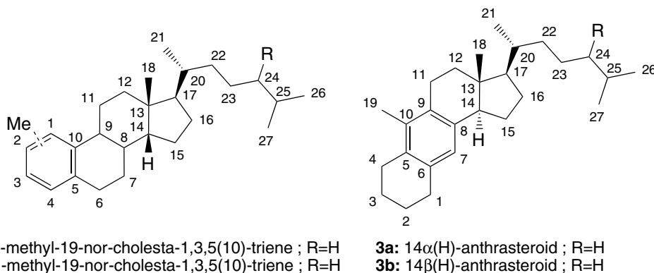
Fig. 2. Sedimentary ring A and ring B monoaromatic steroids.
