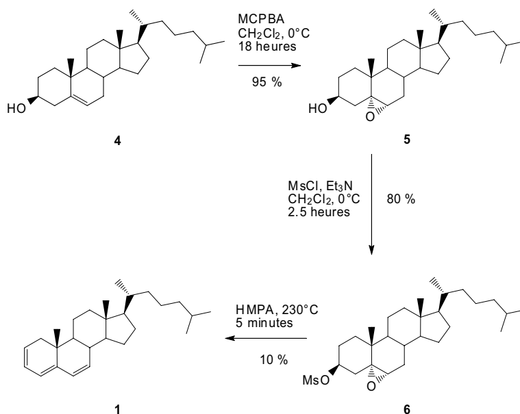
Fig. 3. Preparation of cholesta-2,4,6-triene (1). MCPBA = meta -chloroperbenzoic acid, MsCl = methanesulfonyl chloride and HMPA = hexamethylphosphoramide.
