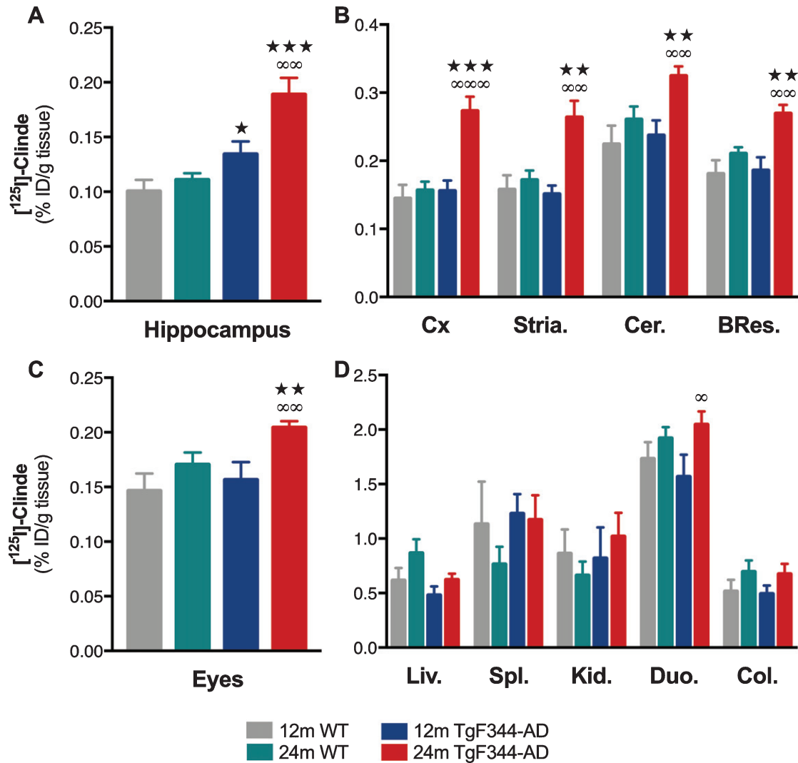
Fig. 1. TSPO overexpression in the brain and in peripheral organs in TgF344-AD rats. The ex vivo measures of [ ^{125} I]CLINDE concentrations (% injected dose -ID-/g of tissue) were performed in the hippocampus (A), in various brain areas (B), in the eyes (C), and in various peripheral organs (D) in wild-type (WT) and TgF344-AD rats at the age of 12 and 24 months. [ ^{125} I]CLINDE concentrations were analyzed by two-way ANOVA. Post hoc tests indicate genotype differences at the same age (★) and age effects in TgF344-AD (∞). The number of symbols indicates the significance level (1: p < 0.05 ; 2: p < 0.01 ; 3: p < 0.001 ). Mean \pm SEM of 8 animals per genotype and per age are presented. BRes., brain residue; Cer., cerebellum; Col., colon; Cx, frontal cortex; Duo., proximal duodenum; Kid., kidney; Liv., liver; Spl., spleen; Stria., striatum.
