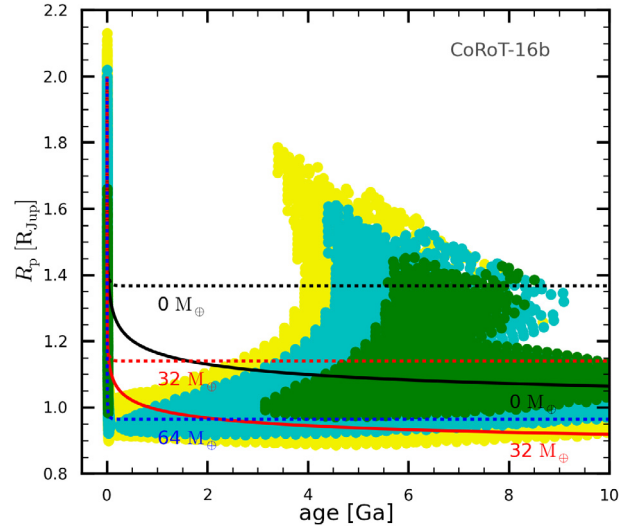
Fig. 11. Constraints obtained on the age (in billions of years) and radius of CoRoT-16b (radius in Jupiter units). The colored circles correspond to stellar models solutions that match the inferred \rho_{\star} - T_{\text{eff}} uncertainty ellipse within 1\sigma (green), 2\sigma (blue), or 3\sigma (yellow). The evolution tracks show the contraction of a 0.535 M_{\text{Jup}} planet with T_{\text{eq}} \sim 1200 \text{ K} , in the so-called “standard approach” (plain lines), and when dissipating 0.25% of the incoming stellar flux, or about 2.6 \times 10^{26} \text{ erg s}^{-1} at the center (dashed lines). The line colors correspond to different masses of the planetary rocky core: 0 M_{\oplus} (black), 32 M_{\oplus} (red), and 64 M_{\oplus} (blue).
