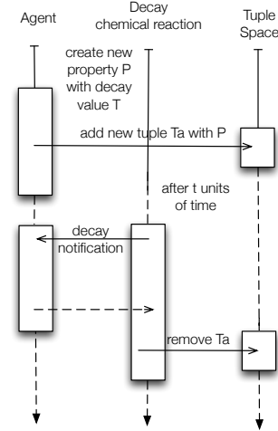
Figure 3: The decay chemical reaction.
