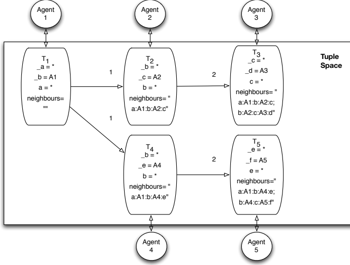
Figure 5: An instance of the tuple space at the end of the discovery process. Solid lines point out bonds between tuples of services during the reading of their property “neighbour”. Edge labels define instants of time when tuples are created/activated.
