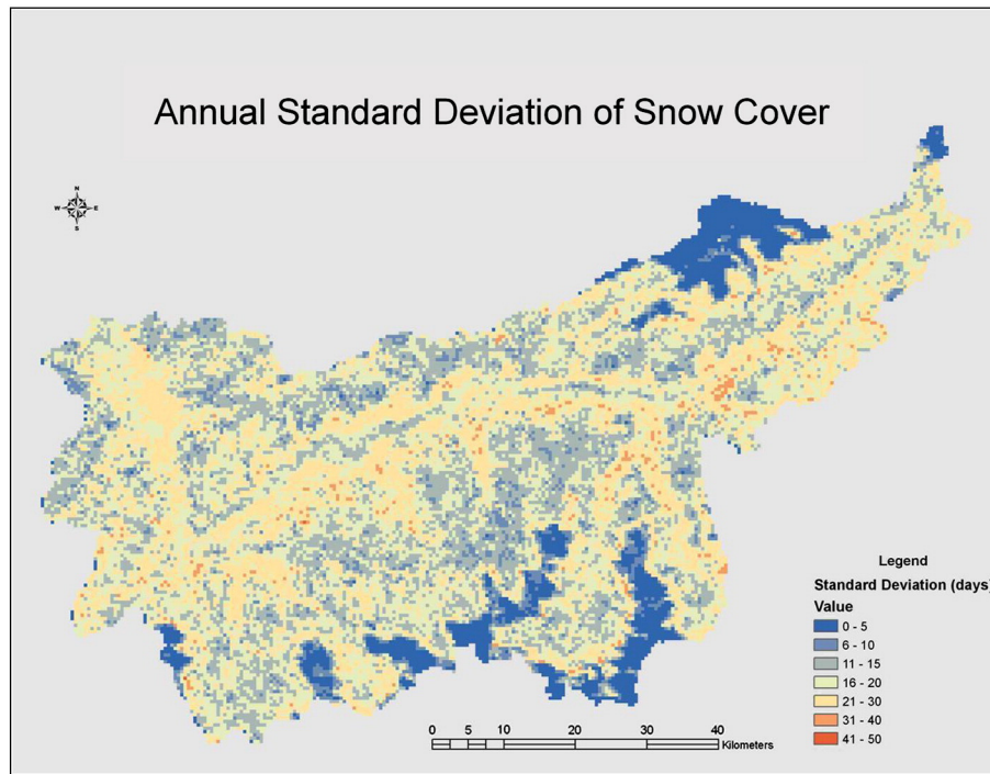
Fig. 11. Annual standard deviation of snow cover (days) for the period 2000–2010, for the upper Rhone watershed. In blue are the glaciated areas with regular snow regime. (For interpretation of the references to color in this figure legend, the reader is referred to the web version of this article.)
