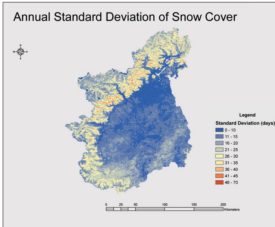
Fig. 12. Annual standard deviation of snow cover (days) for the period 2000–2010, for the upper Po watershed. In red are the foothills of Piedmont with non-inter-annual regular snow regime. (For interpretation of the references to color in this figure legend, the reader is referred to the web version of this article.)
