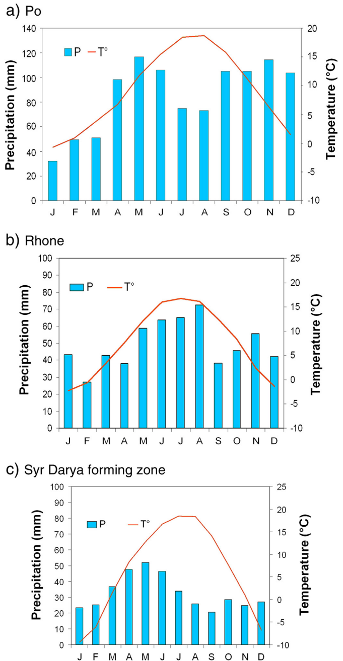
Fig. 7. Monthly average distribution of precipitation and temperature (2001–2010) for: (a) Po, (b) Rhone, and (c) upper Syr Darya watersheds.
