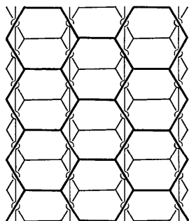
Fig. 2. Schematic representation of the structure slab building up the \text{Al}_2\text{Cu} , \text{Mg}_2\text{Cu} and \text{Mg}_2\text{Ni} structure types. The hexagonal nets indicate edges of square antiprisms of Al or Mg atoms that can be shared with those of the neighbouring slabs below (thin lines) and above (thick lines). Rows of open circles indicate Cu or Ni atoms that centre chains of square antiprisms.
