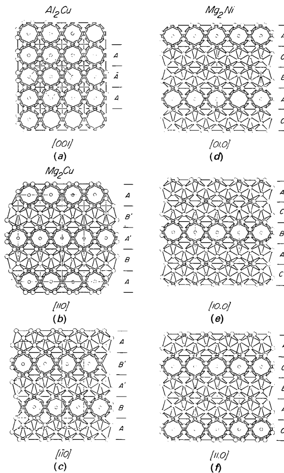
Fig. 1. The structures of (a) tetragonal Al 2 Cu along [001]; orthorhombic Mg 2 Cu along (b) [110] and (c) [110]; and hexagonal Mg 2 Ni along (d) [01.0], (e) [10.0] and (f) [11.0].
