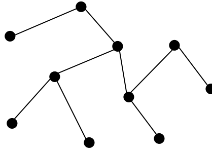
Figure 1.b: Example of a tree.
