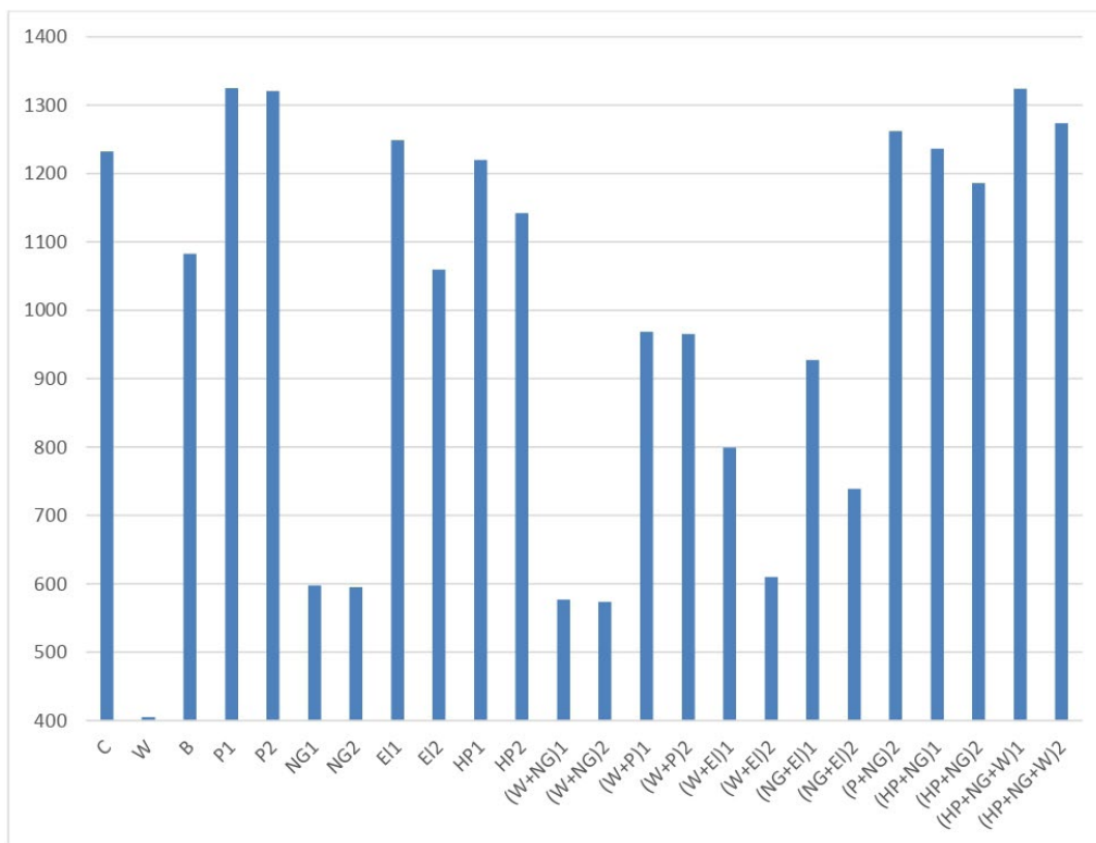
Fig. 2. Household total costs for the heating system operation under different options of energy carriers and their combinations used during the heating season [EUR] (explanations for the heating options codes are provided in Tables 5 and 6)
