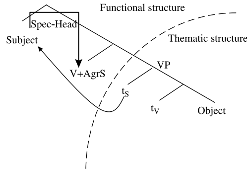
Fig. 3. Late stages of the derivation.
