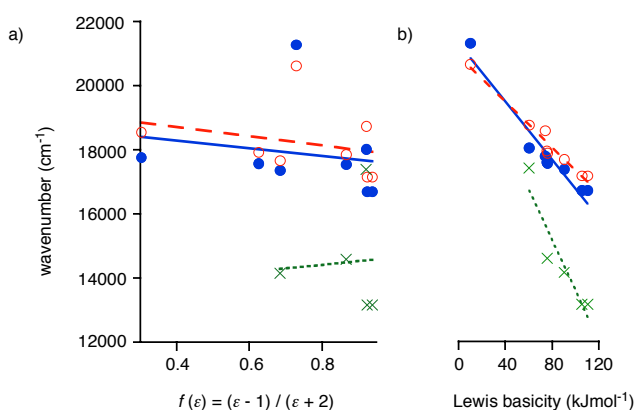
Fig. 7. Absorption maxima of 9 (●), 10 (○) and 11 (X) in wavenumbers as a function of (a) the polarity function f(\epsilon) and (b) -\Delta H_0^{\text{BF}_3} (295.15), the Lewis basicity of the solvent.
