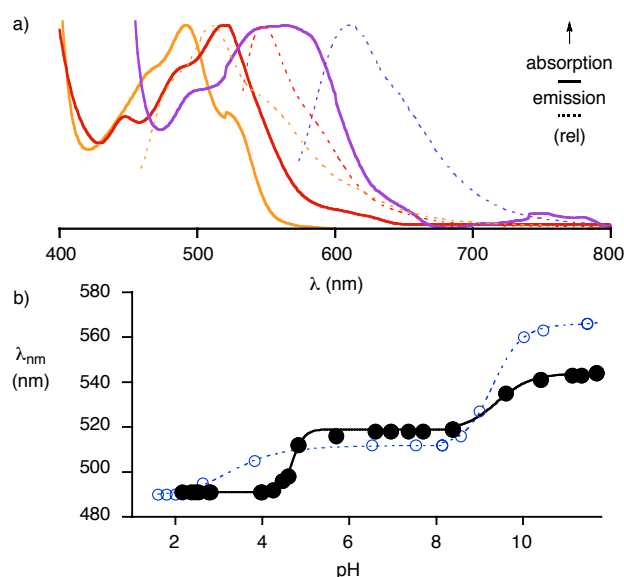
Fig. 10. a) Absorption (solid) and emission (dotted) spectra of 22 (pH 3, orange), 24 (pH 7, red) and 25 (pH 11, violet) in DMSO/water 4:1, 25 °C. b) Absorption maxima of 22 (●) and 10 (○) as a function of pH.
