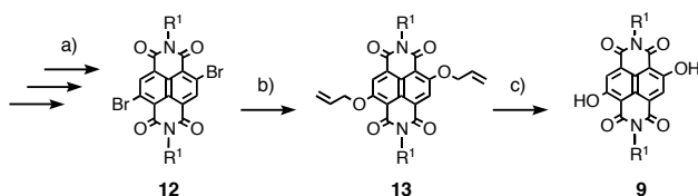
Scheme 1. Synthesis of cNDI 9 with a hydroquinone core. a) Naphthalenedianhydride, several reported steps. 16 b) Allyl alcohol, NaH, dichloromethane, 4 Å MS, 4 h, rt, 86%. c) Pd(PPh 3 ) 4 , phenylsilane, dichloromethane, 4 Å MS, 10 h, rt, 80% (R 1 = mesityl).
