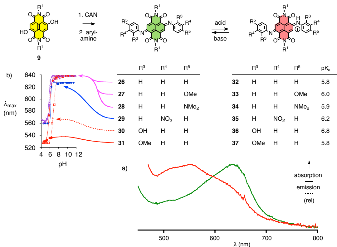
Fig. 11. a) Absorption spectra of 26 (pH 9, green) and 32 (pH 4, red) in DMSO/water 4:1, 25 °C. b) Change in absorption maxima of imines 26-31 upon protonation with decreasing pH to give iminium cations 32-37 .
