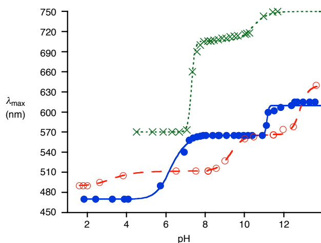
Fig. 4. Absorption maxima of 9 (●), 10 (○) and 11 (X) as a function of pH.
