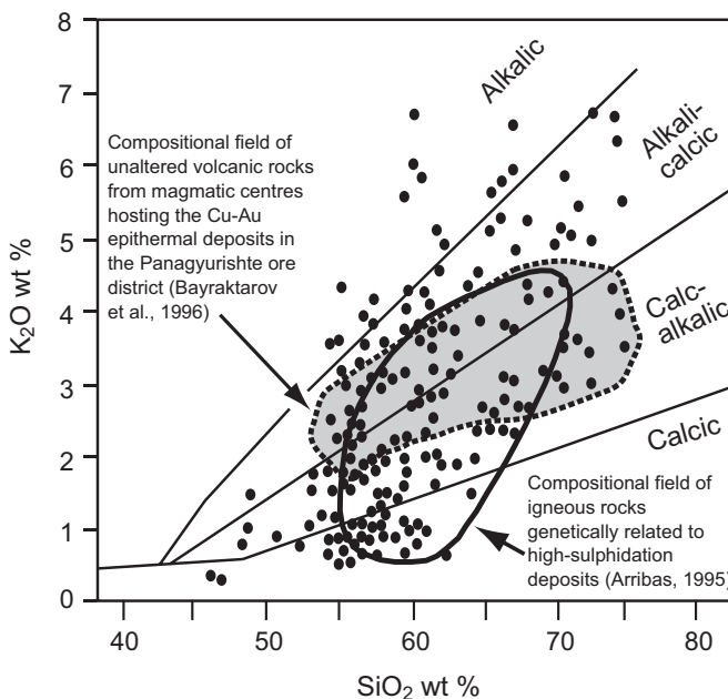
Fig. 2 K_2O vs. SiO_2 diagram for Late Cretaceous igneous rocks from the Panagyurishte ore district (black dots). Data for the Panagyurishte ore district from Bayraktarov et al. (1996), and data compilation of igneous rocks genetically related to high-sulphidation deposits from Arribas (1995).
