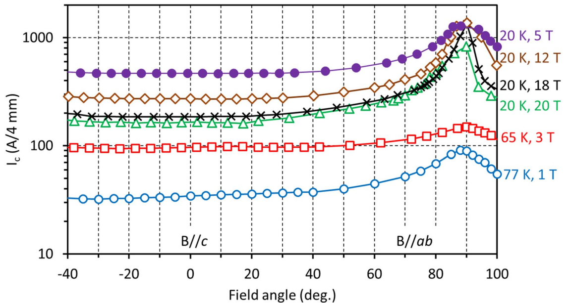
Figure 2. Angular dependences of I_c in magnetic field of YBCO wire at 77 K, 1 T; 65 K, 3 T and 20 K, 5, 12, 18, and 20 T. Measurements were performed at Tohoku University. 0° corresponds to the B/c orientation and 90° corresponds to the B/ab orientation. Within the accuracy of measurement, the minimum value of I_c for all field orientations is at B/c . At 20 K, I_c at B/ab stays almost constant with increasing magnetic field. We believe the smaller value of I_c at B/ab at 20 T may be an artefact due to the sharp I_c angular peak and the discrete angle step during measurements.
