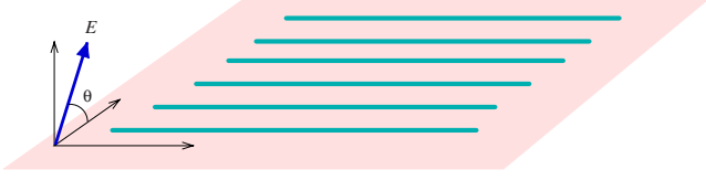
FIG. 1. (Color online) Array of one-dimensional chains formed by a two-dimensional optical lattice. The polarizing field E is directed perpendicular to the chains and at an angle \theta which can be used to tune the interchain interaction V_{\perp} in (2).
