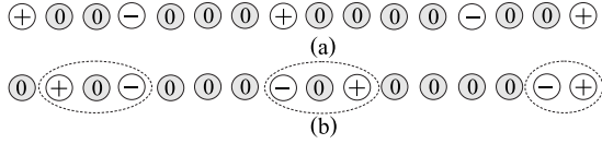
FIG. 2. Typical configurations in the (a) HI and (b) MI ground states. The numbers represent \delta n_i (the deviation of the local occupation from the average density). The HI can be described as a charge ordered +, -, +, \dots state with an undetermined number of 0 sites between each + and - . The MI is a dilute gas of particle-hole pairs (indicated by the dotted line).
